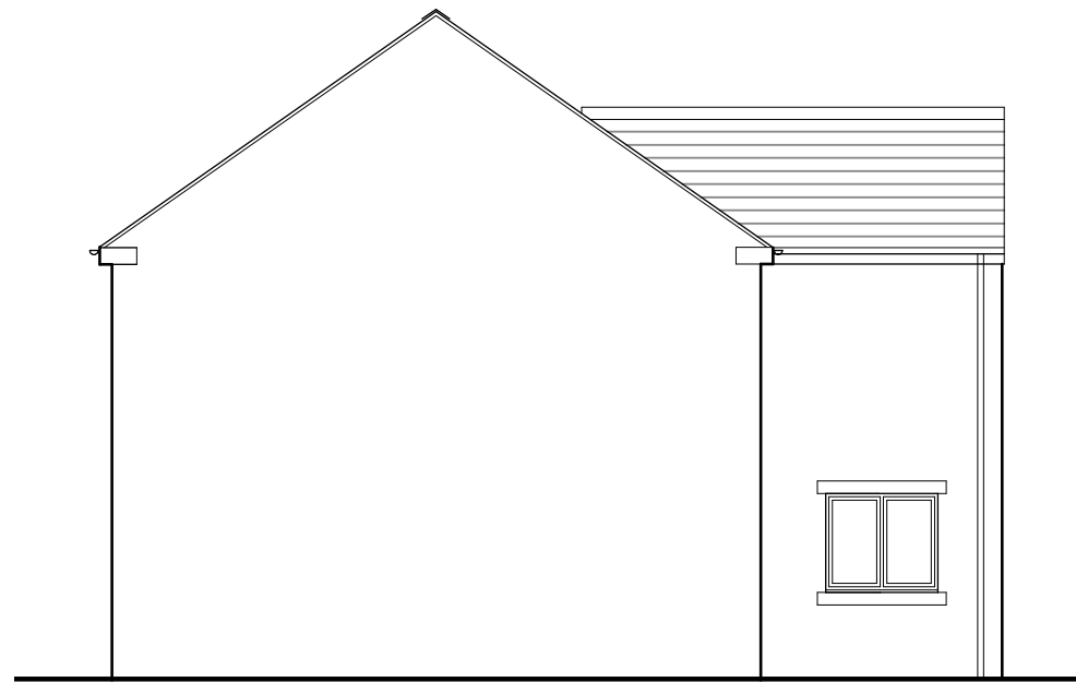
House 1 and 3- South Elevation
